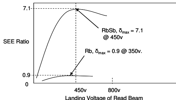
Figure 10. Rb over RbSb Media layers
