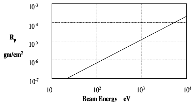
Figure 7. Practical Range R_p vs. Beam Energy
