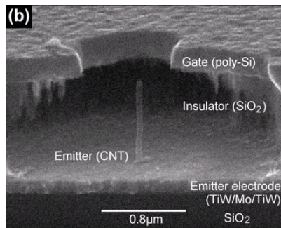
Figure 3. CNT Emitter in Gated Cavity
