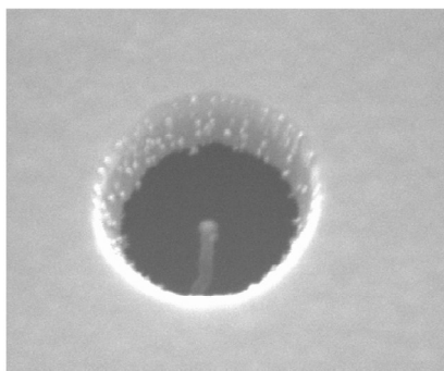
Figure 4. SEM Photo of CNT Gated Emitter with 800nm Diameter Cavity.
