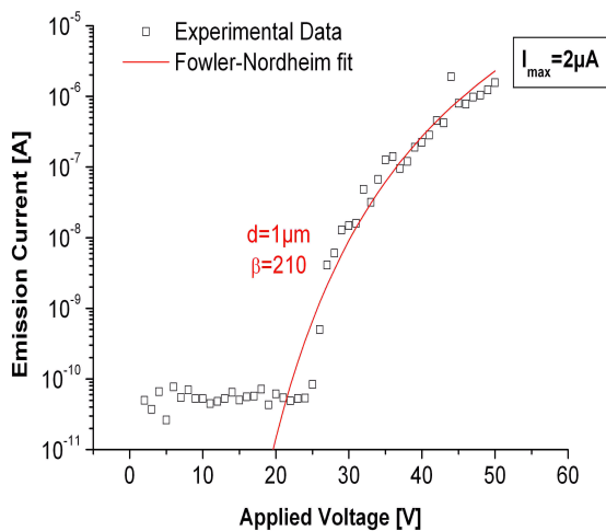
Figure 5. CNT Emitter Current vs. Voltage
