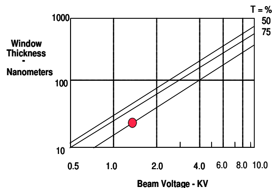
Figure 8. Silicon Nitride Window, Transmission vs. Thickness & Beam Energy
