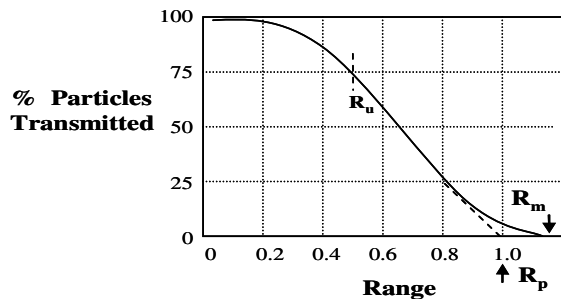
Figure 6. Particle Transmission Ranges
