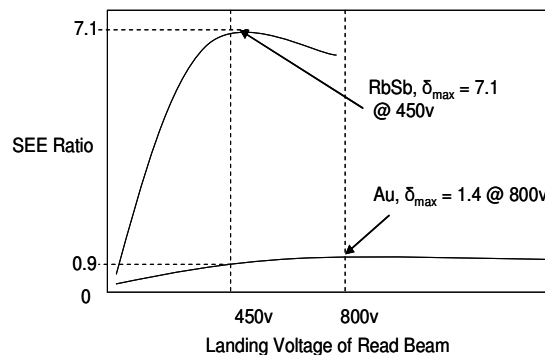
Figure 9. SEE Response Curves for RbSb / Gold Archival media
