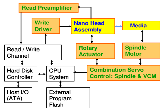
Figure 2. Typical Disk Drive Configuration.
