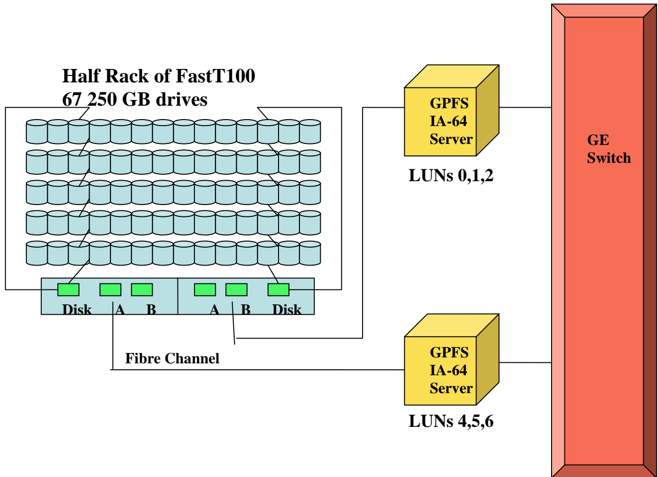
Figure 2. 1/32 of the disk and server arrangement
