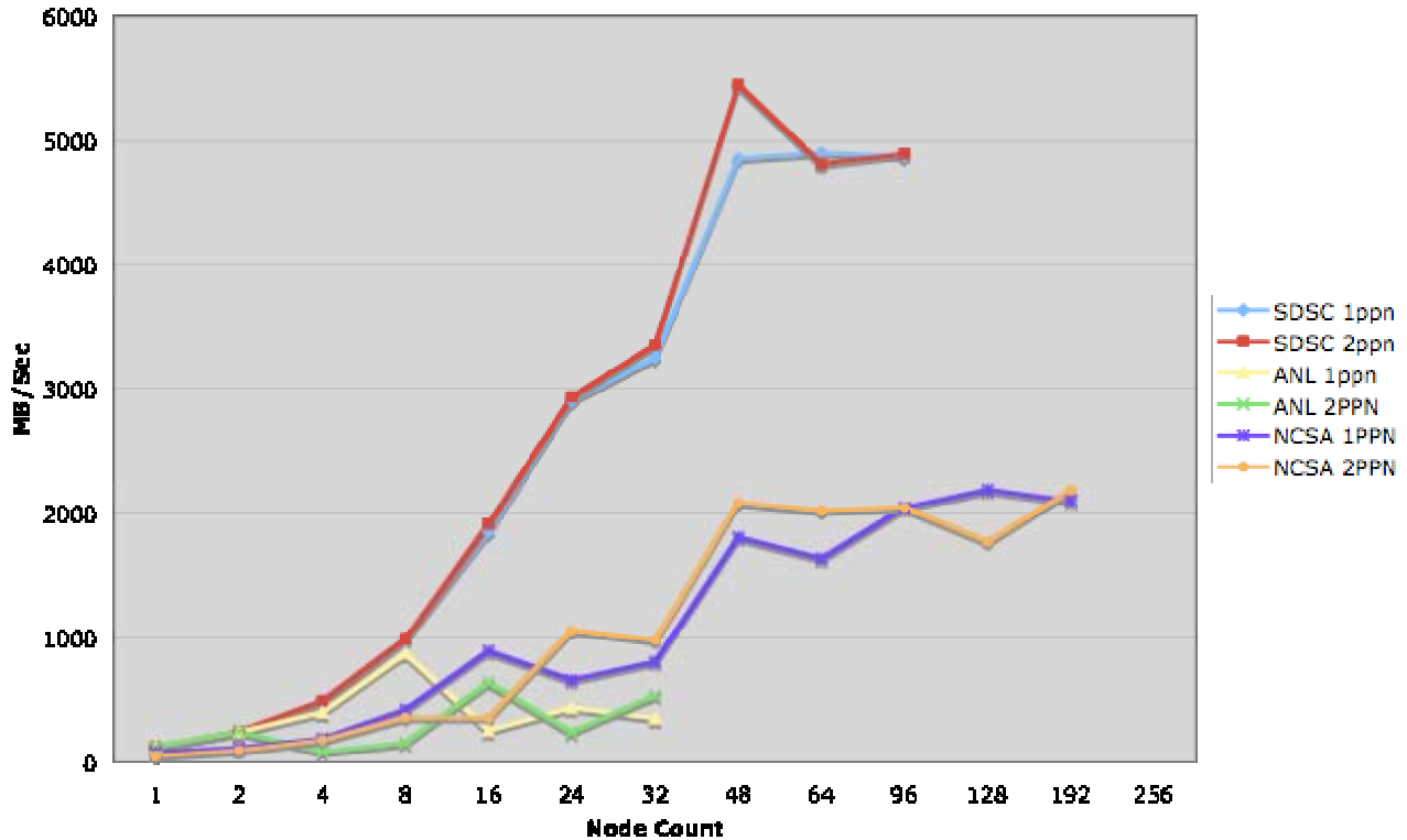
Figure 4. GPFS-WAN Write Performance in MB/S, 1 & 2 processes per node
