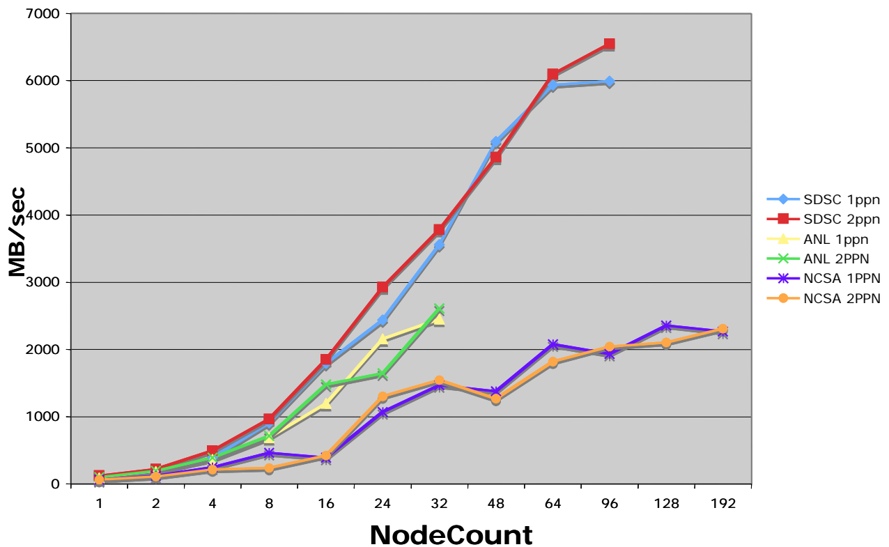
Figure 3. GPFS-WAN Read Performance in MB/S, 1 & 2 processes per node
