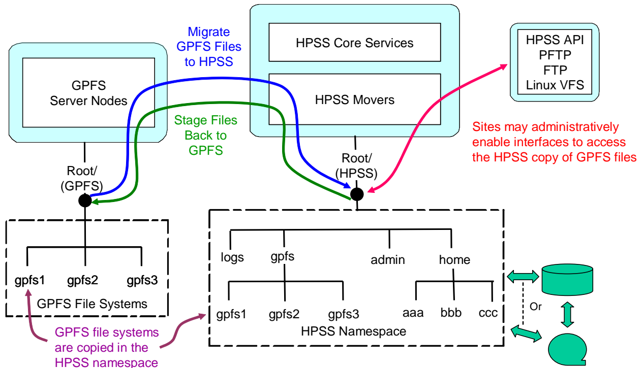
Figure 9. GPFS-HPSS integration diagram
