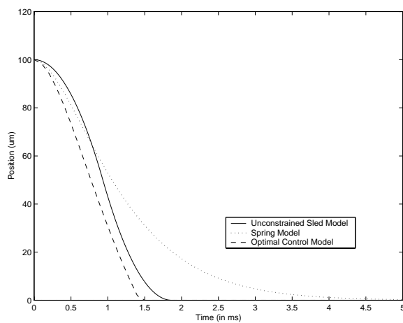
Figure 4: Model dynamics.
