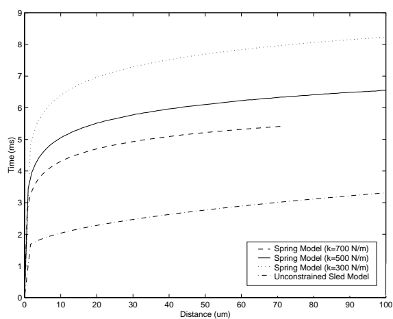
Figure 8: Changing the spring constant.
