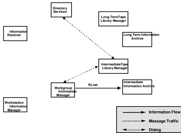
Figure 6. Information Migration Process
