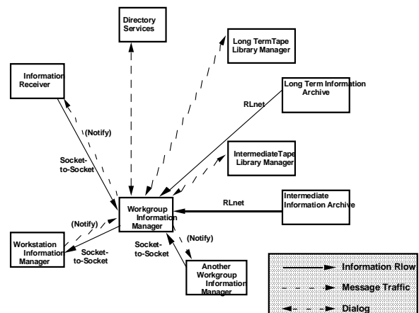
Figure 5. Information Pull Process
