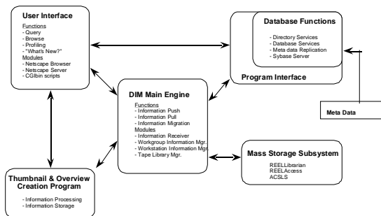
Figure 3. Pilot Software: Logical Architecture
