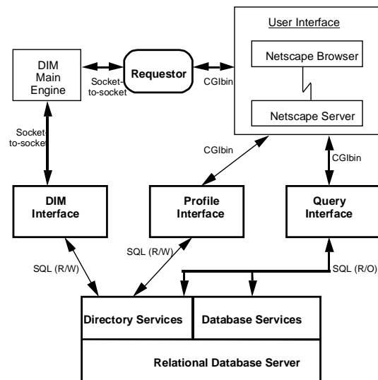
Figure 7. Anatomy of Database Subsystem
