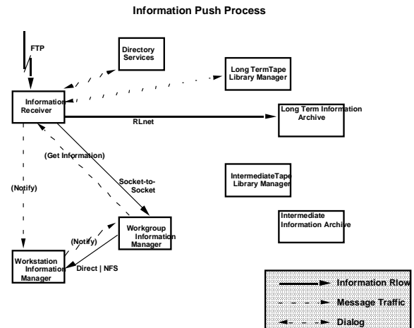
Figure 4. Information Push Process
